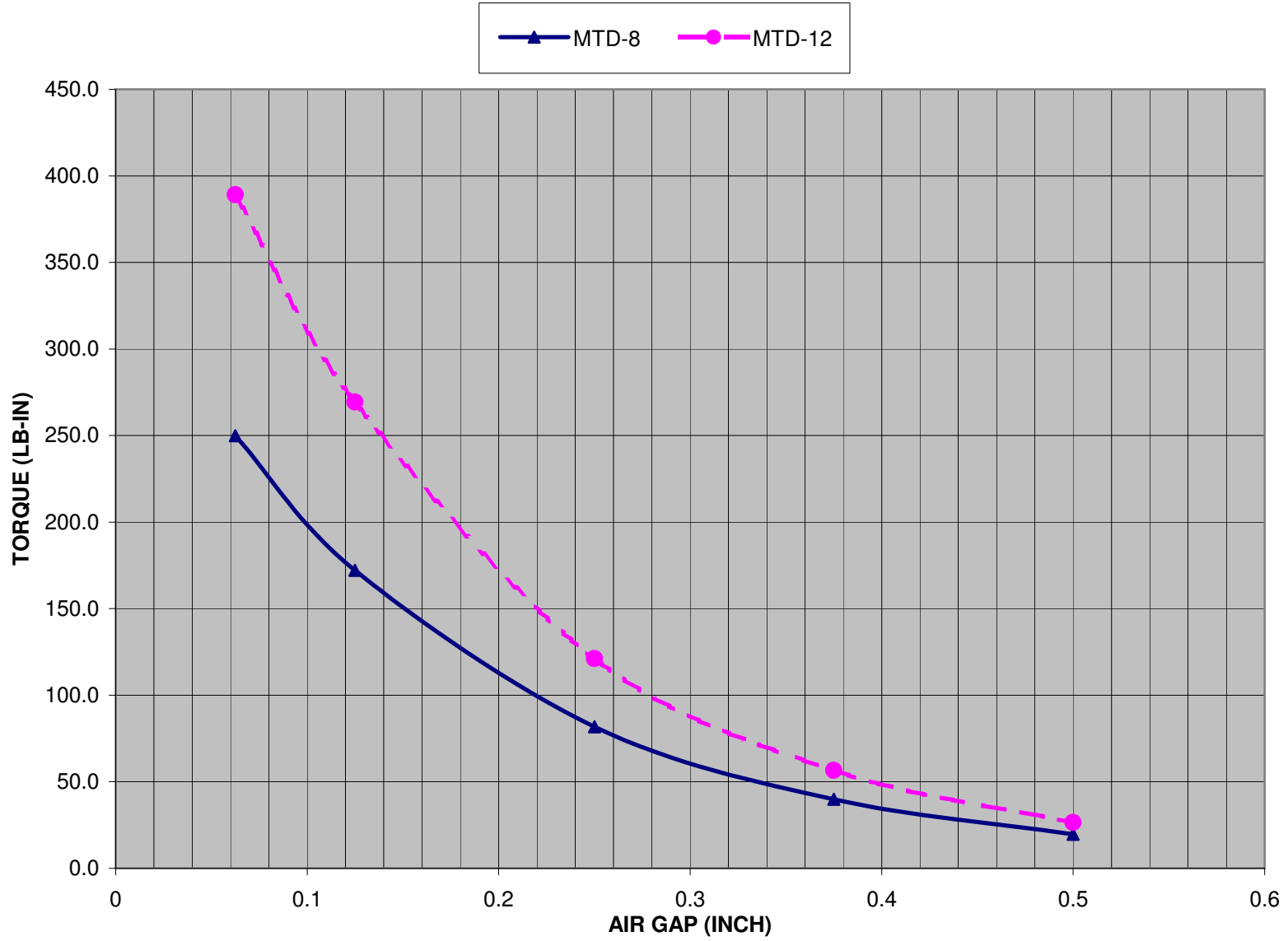
MTD 8 & 12 TORQUE VS AIR GAP
