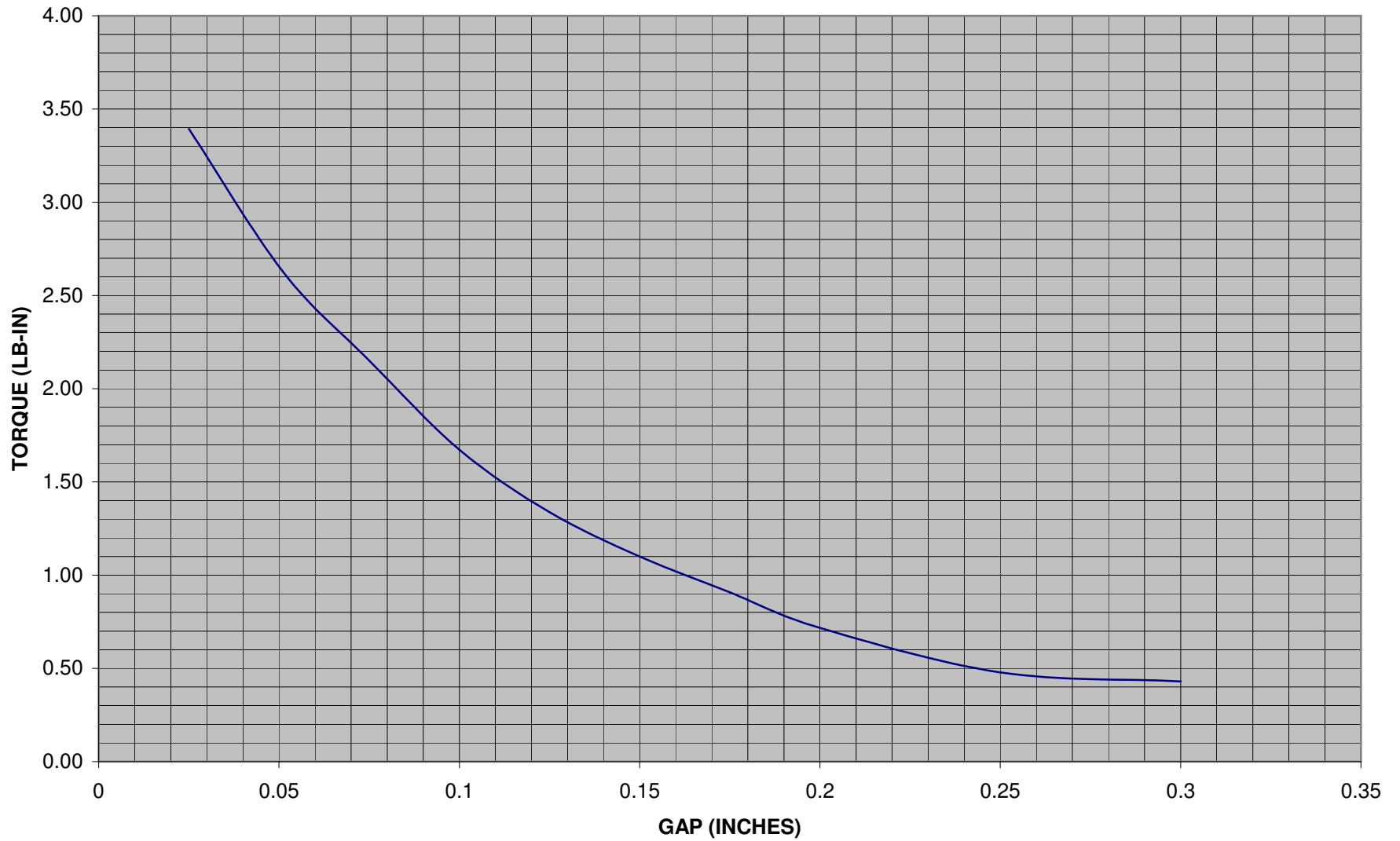
MTD-0.2 GAP VS TORQUE 5-20-2010
